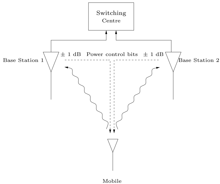
Figure 4.6: Soft handoff.
