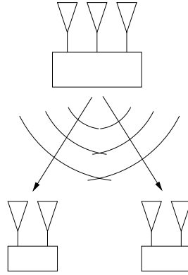
Figure 10.29: The downlink with multiple transmit antennas at the base station and multiple receive antennas at each user.
