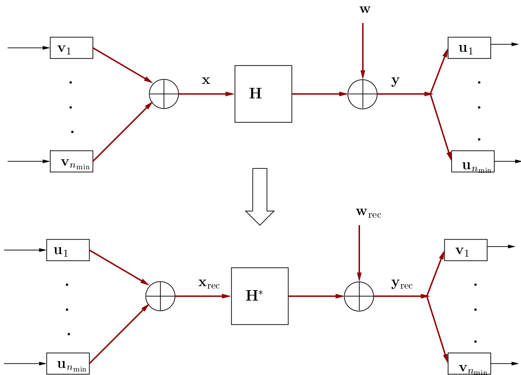
Figure 10.32: The data streams being transmitted and received via linear filters on the primal (top) and reciprocal (bottom) channels.
