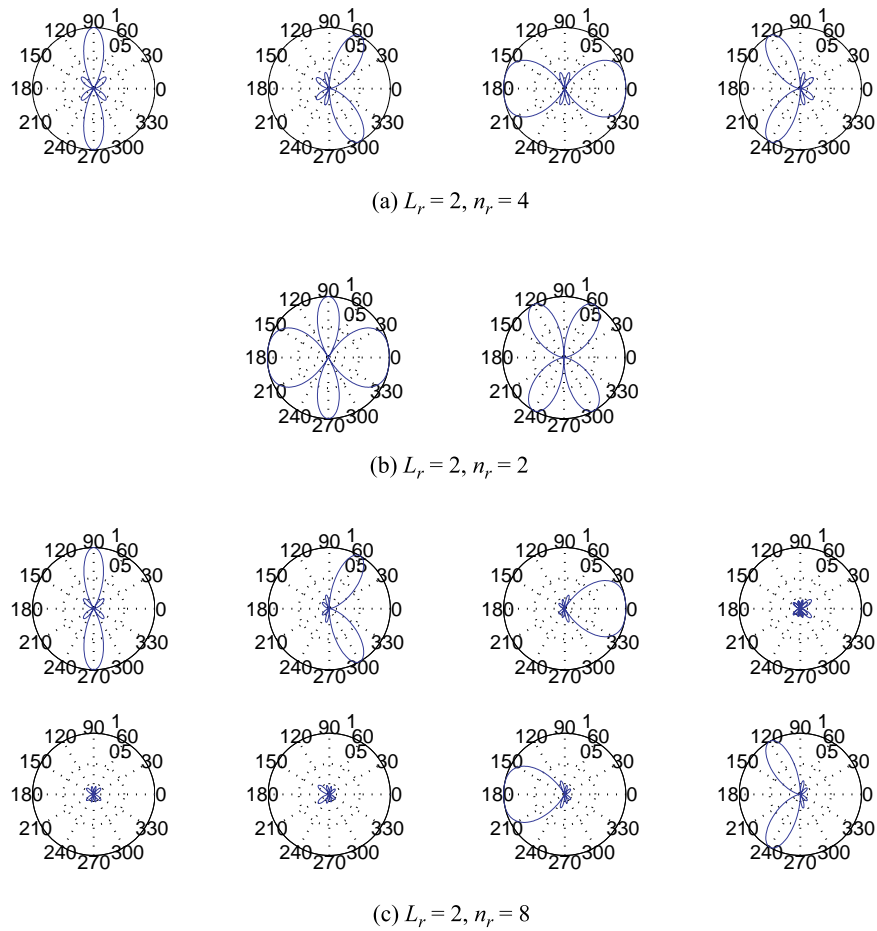
Figure 7.13: Receive beamforming patterns of the angular basis vectors. Independent of the antenna spacing, the beamforming patterns all have the same beam widths for the main lobe, but the number of main lobes depends on the spacing. (a) Critically-spaced case; (b) Sparsely-spaced case. (c) Densely-spaced case.
