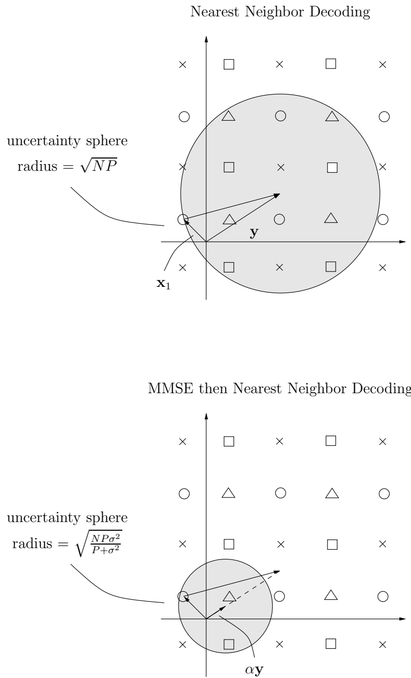
Figure 10.23: MMSE decoding yields a much smaller uncertainty sphere than that by nearest neighbor decoding.
