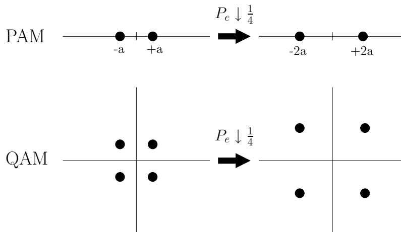
Figure 9.2: Increasing the SNR by 6dB decreases the error probability by 1/4 for both PAM and QAM due to a doubling of the minimum distance.
