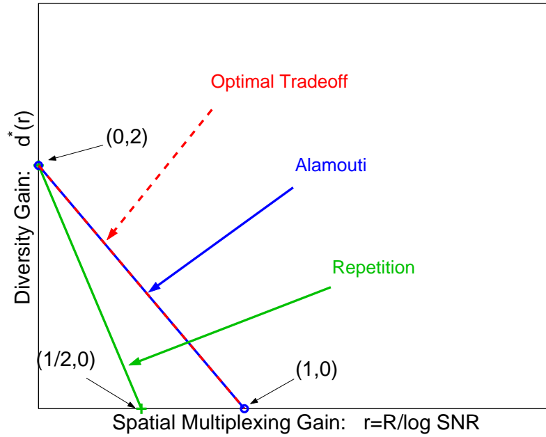
Figure 9.5: The diversity-multiplexing tradeoffs of the 2 \times 1 i.i.d. Rayleigh fading MISO channel together with those of two schemes.
