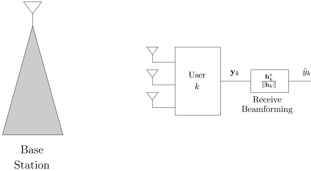
Figure 10.30: Each user with a front end matched filter converting the SIMO downlink into a SISO downlink.
