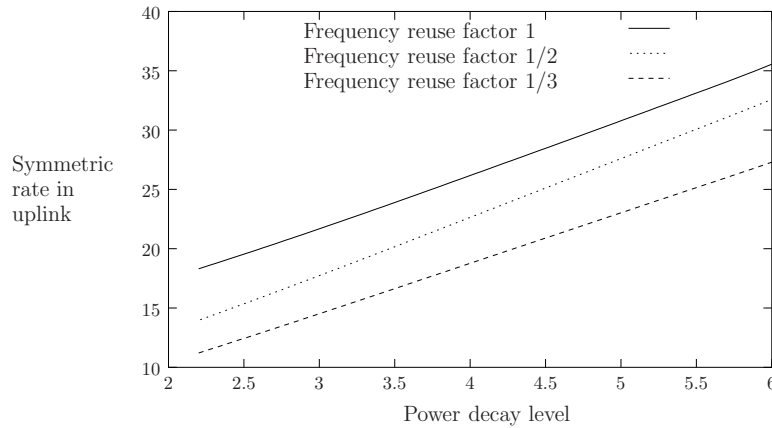
Figure 10.31: The symmetric rate for every user (in bps/Hz) with K = 5 users in SDMA model in an uplink with n_r = 5 receive antennas plotted as a function of the power decay rate \alpha for the linear cellular system. The rates are plotted for reuse ratios 1, 1/2 and 1/3.
