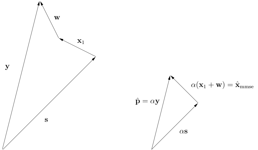
Figure 10.25: The decoding process with the \alpha factor.
