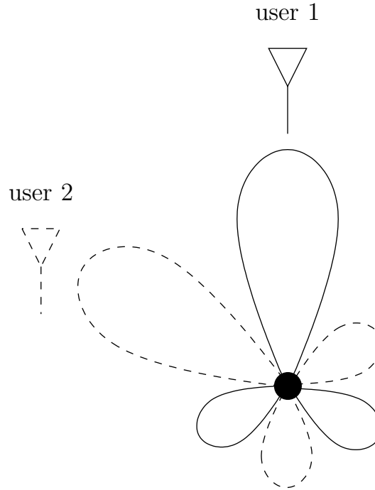
Figure 10.28: Opportunistic beamforming with two orthogonal beams. The user “closest” to a beam is scheduled on that beam, resulting in two parallel data streams to two users.
