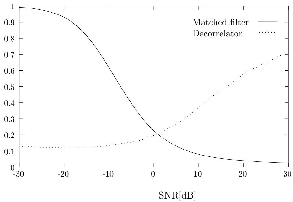
Figure 8.13: Performance (ratio of the rate to the capacity) of the matched filter bank as compared to that of the decorrelator bank. At low SNR, the matched filter is superior. The opposite is true for the decorrelator. The channel is i.i.d. Rayleigh with n_t = n_r = 8 .
