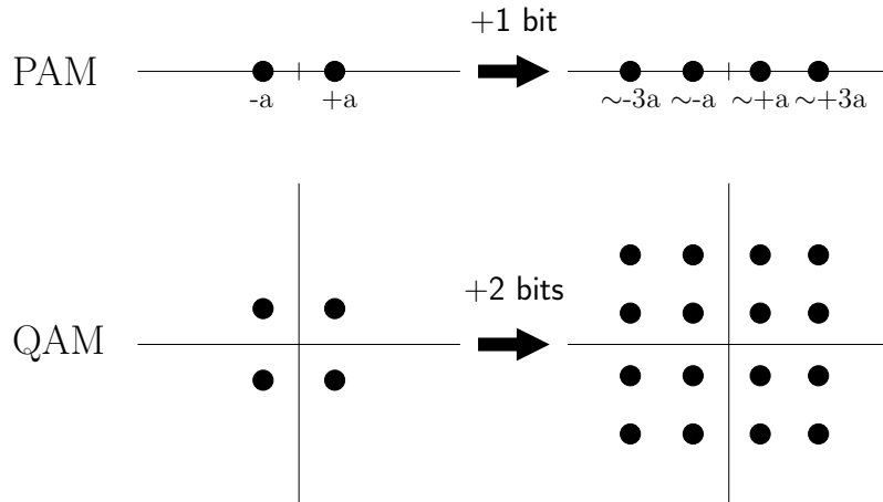
Figure 9.3: Increasing the SNR by 6dB increases the data rate for QAM by 2 bits/s/Hz but only increases the data rate of PAM by 1 bits/s/Hz.
