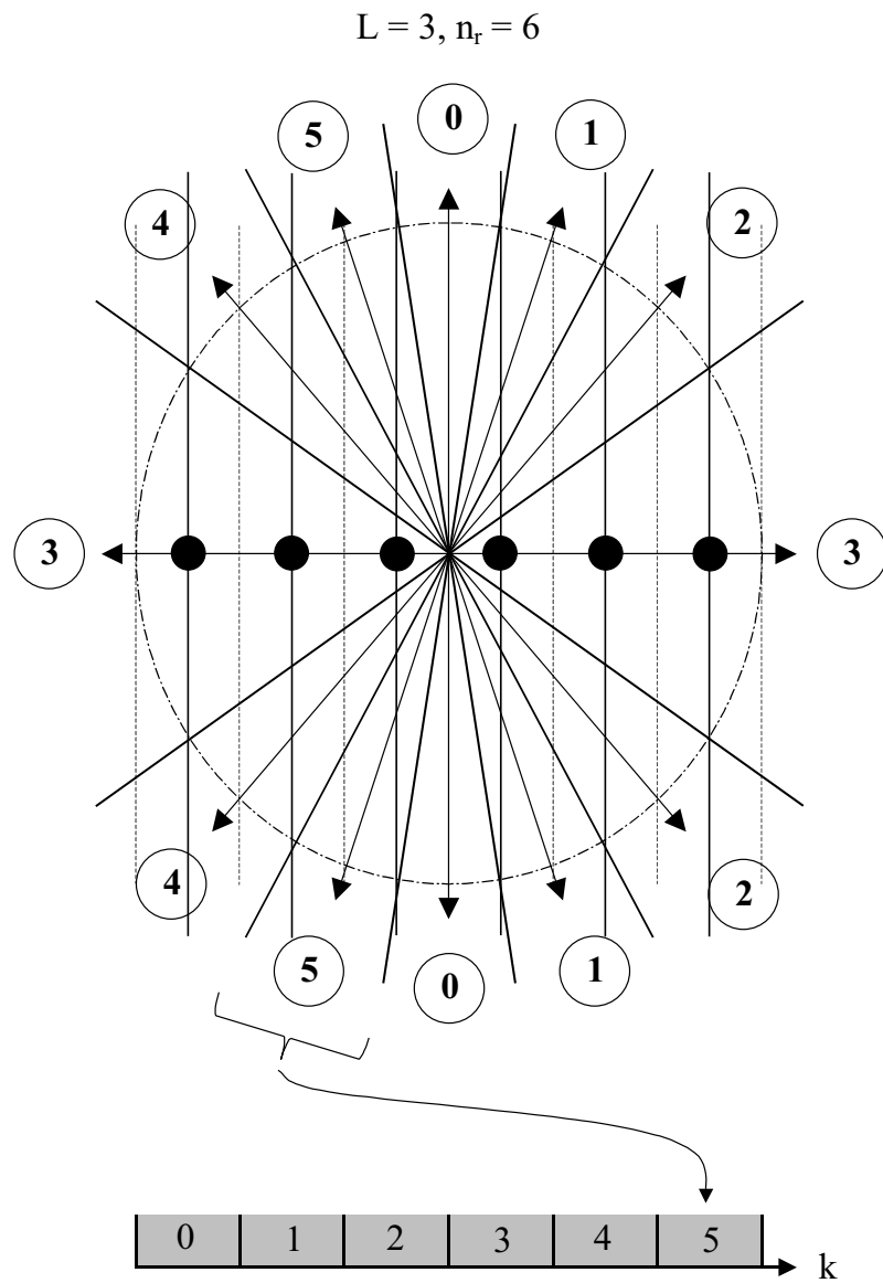
Figure 7.22: Antennas are critically spaced at half the wavelength. Each resolvable bin corresponds to exactly one angular window. Here, there are 6 angular windows and 6 bins.
