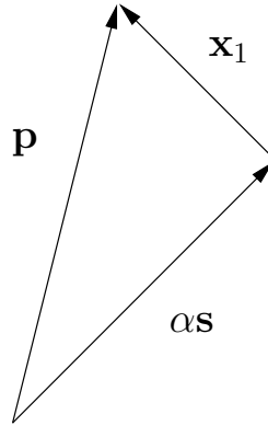
Figure 10.24: The precoding process with the \alpha factor.
