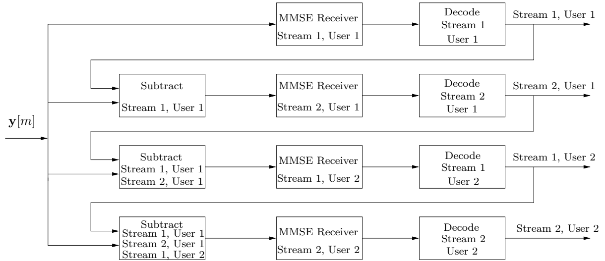
Figure 10.12: Receiver architecture for the two-user MIMO uplink. In this figure, each user has two transmit antennas and split their data into two data streams each. The base station decodes the data streams of the users using the linear MMSE filter, successively canceling them as they are decoded.
