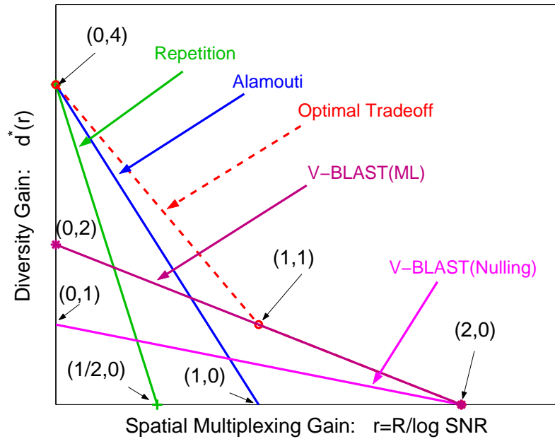
Figure 9.6: The diversity-multiplexing tradeoffs of the 2 \times 2 i.i.d. Rayleigh fading MISO channel together with those of four schemes.
