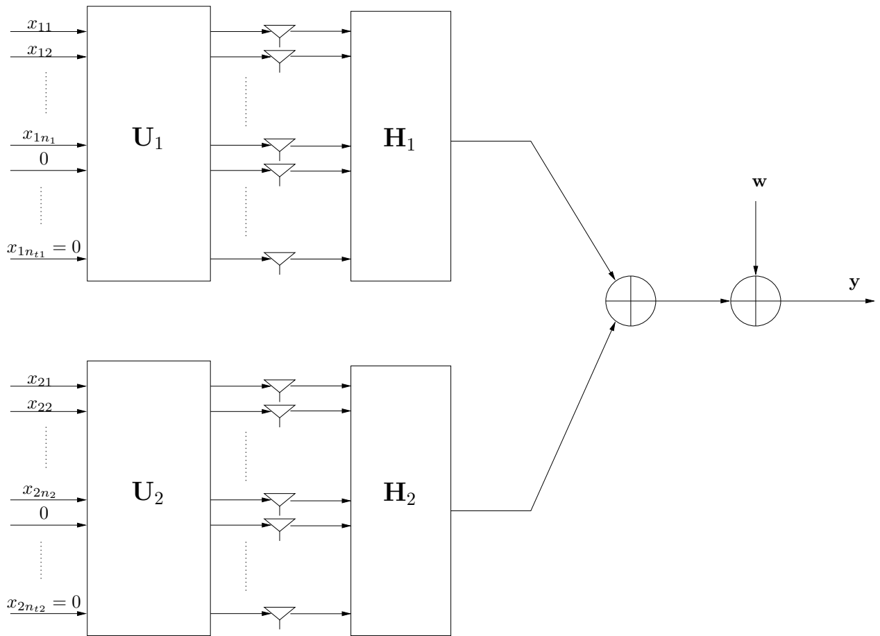
Figure 10.11: The transmitter architecture for the two-user MIMO uplink. Each user splits its data into independent data streams, allocates powers to the data streams and transmits a rotated version over the transmit antenna array.
